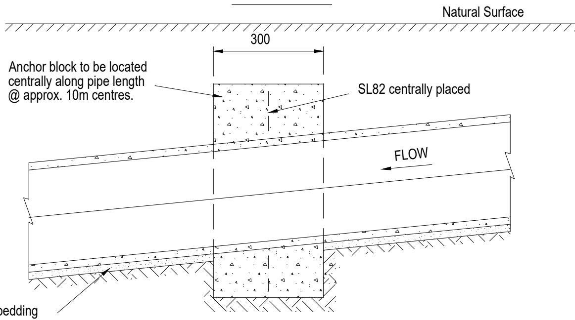
SECTION ALONG PIPE LENGTH
