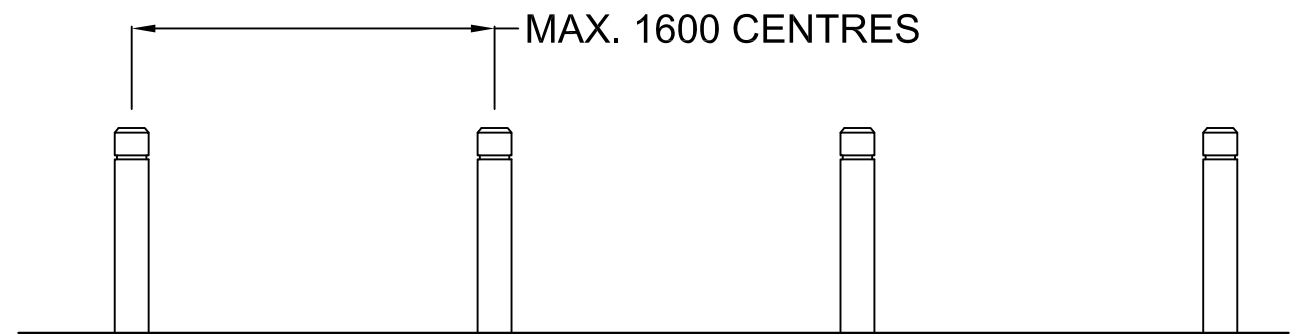
INSTALLATION ELEVATION
